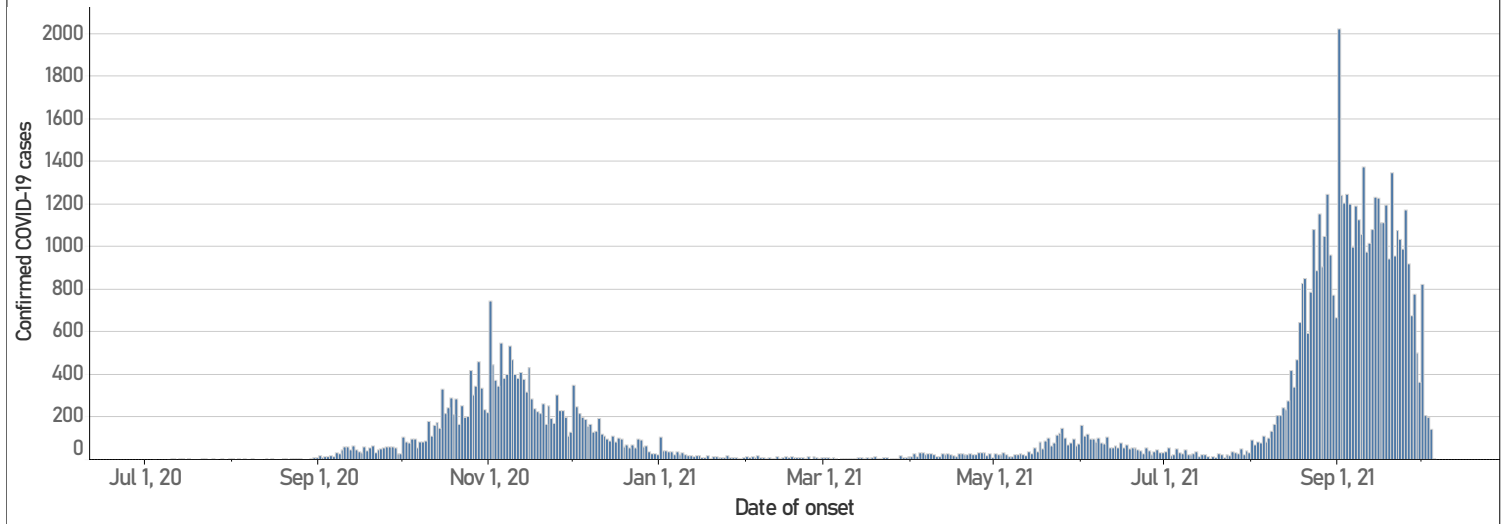
Daily COVID-19 confirmed cases by the lab result date
