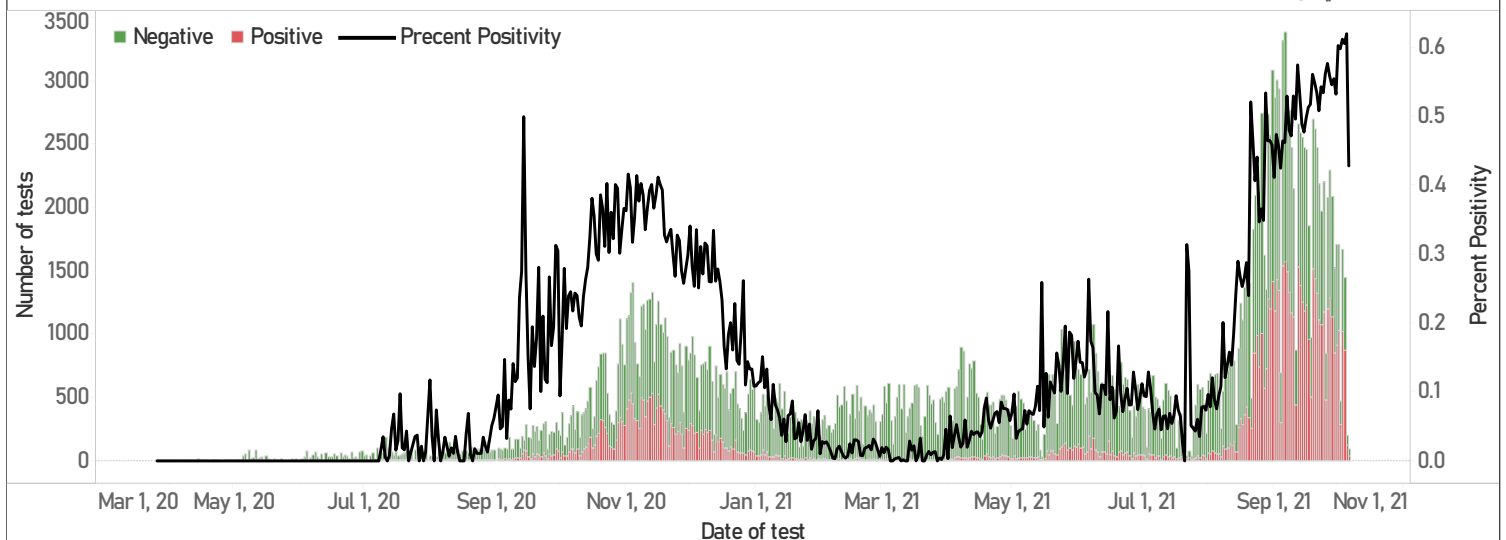
Daily tests and the positivity rate
